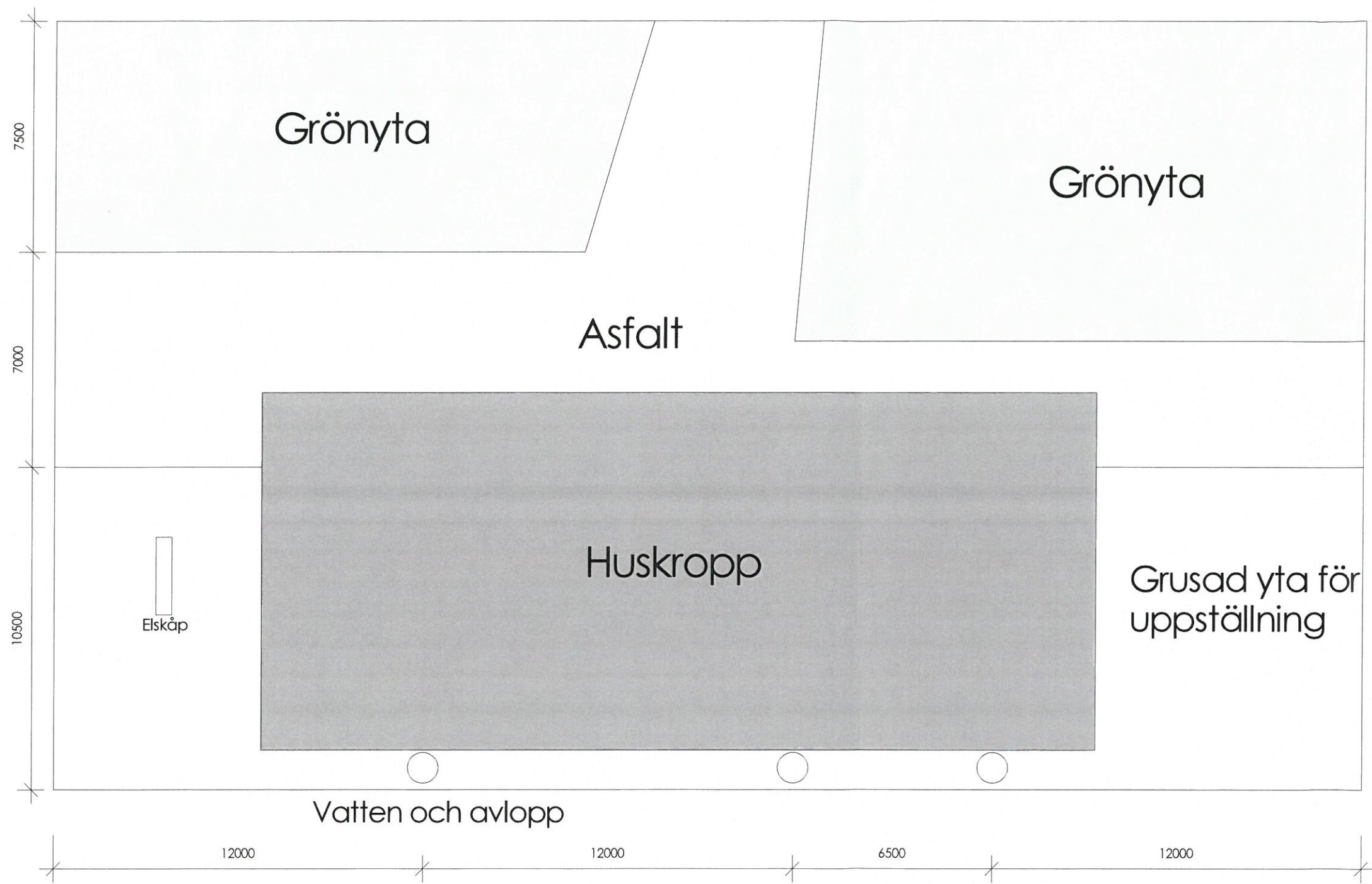
A103 - Situationsplan 1 : 150
